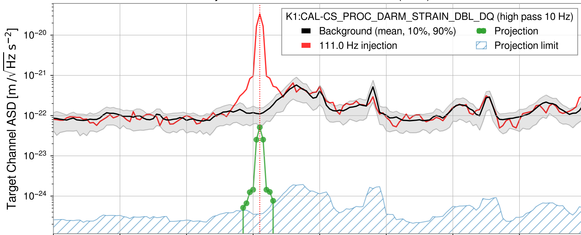
Injection from GPS1428962173.085 (8sec)
