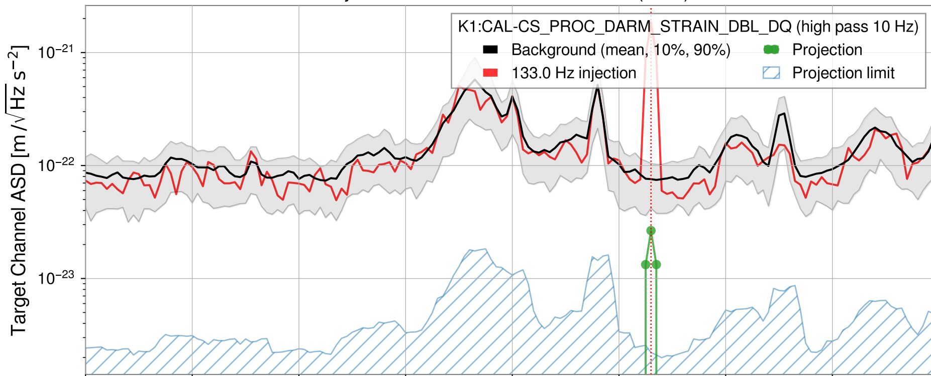
Injection from GPS1428961908.755 (8sec)
