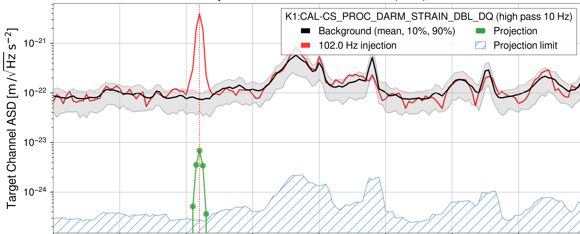
Injection from GPS1428962281.22 (8sec)
