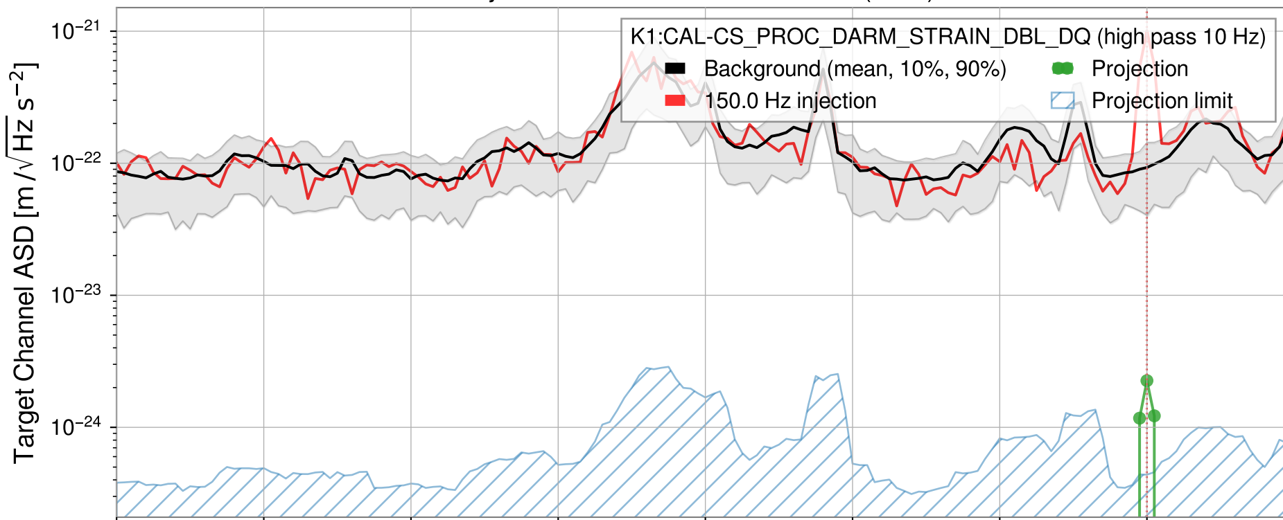
Injection from GPS1428961704.5 (8sec)
