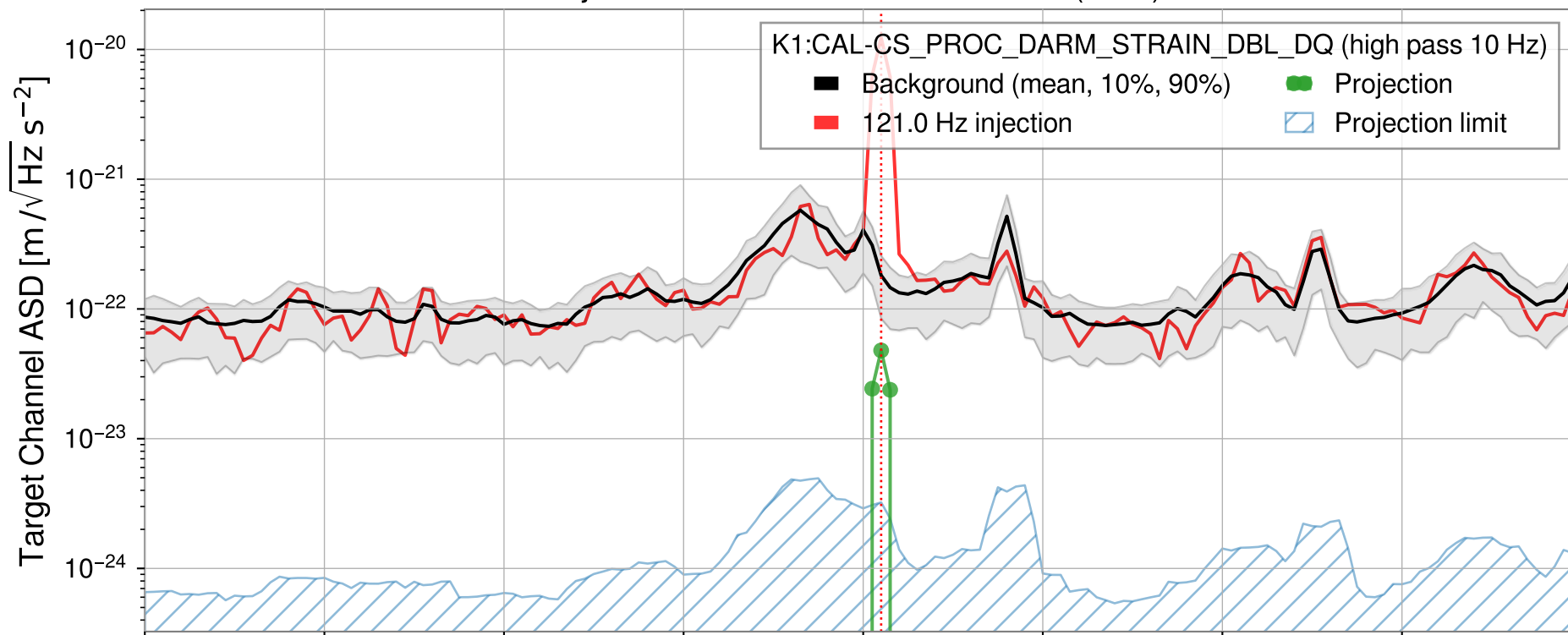
Injection from GPS1428962052.935 (8sec)
