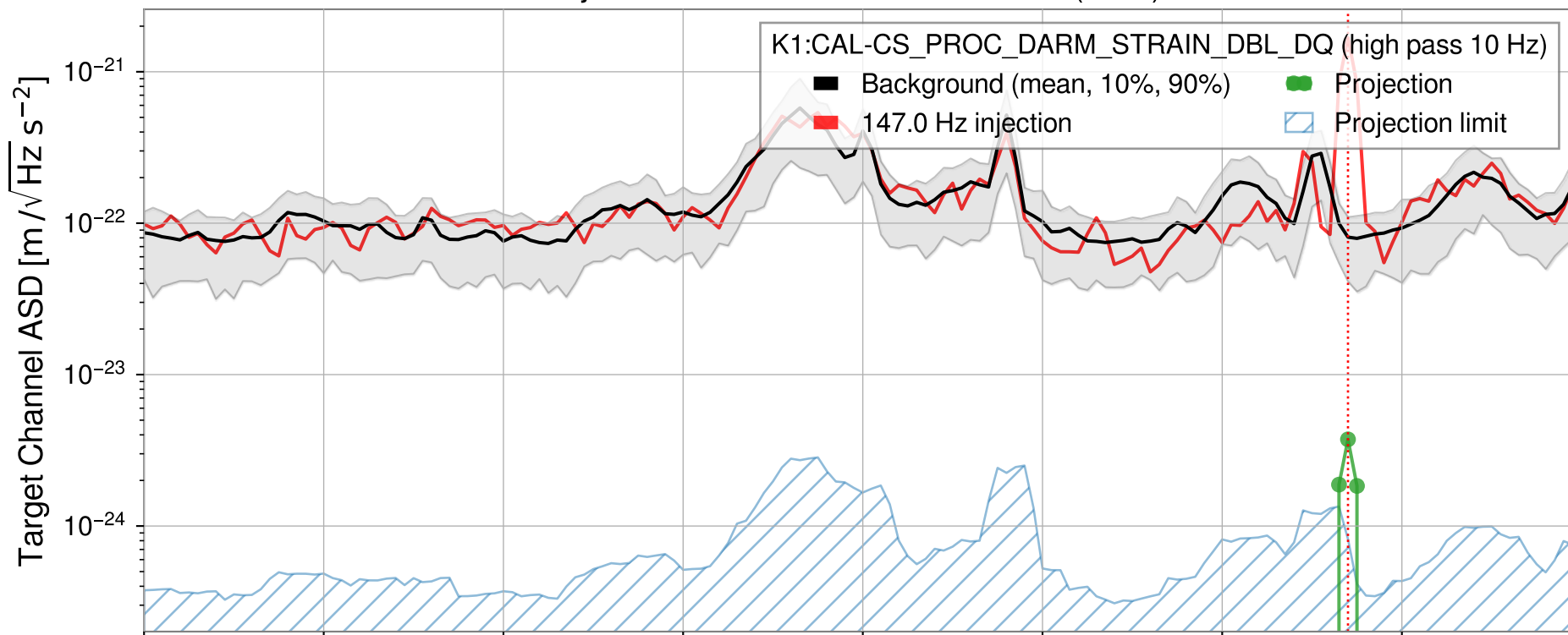
Injection from GPS1428961740.545 (8sec)
