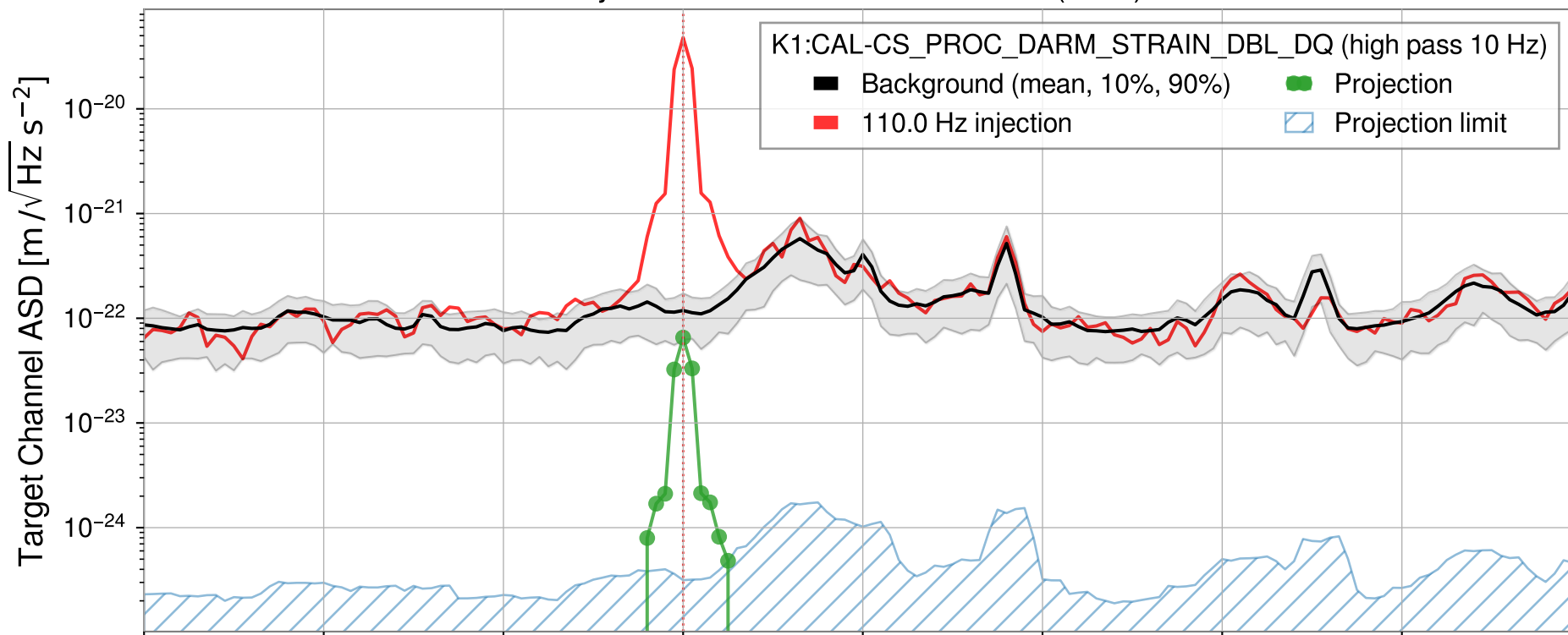
Injection from GPS1428962185.1 (8sec)
