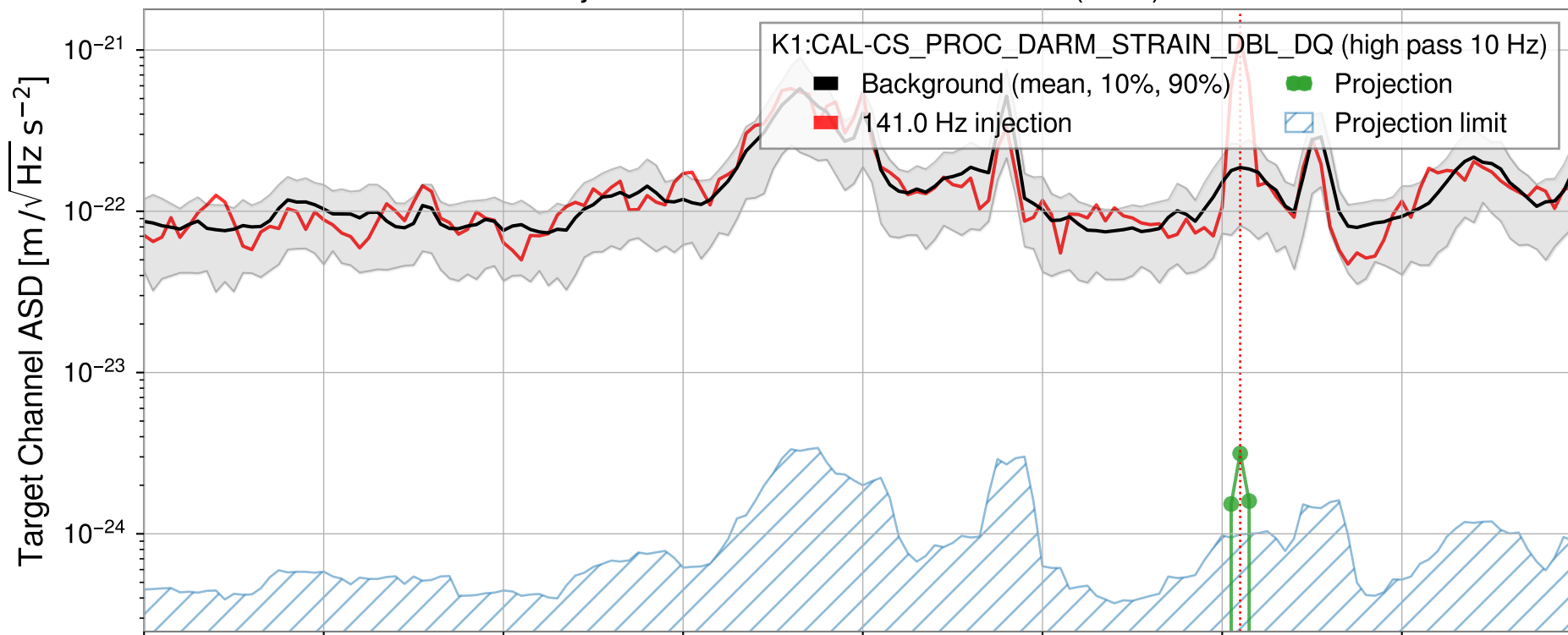
Injection from GPS1428961812.635 (8sec)
