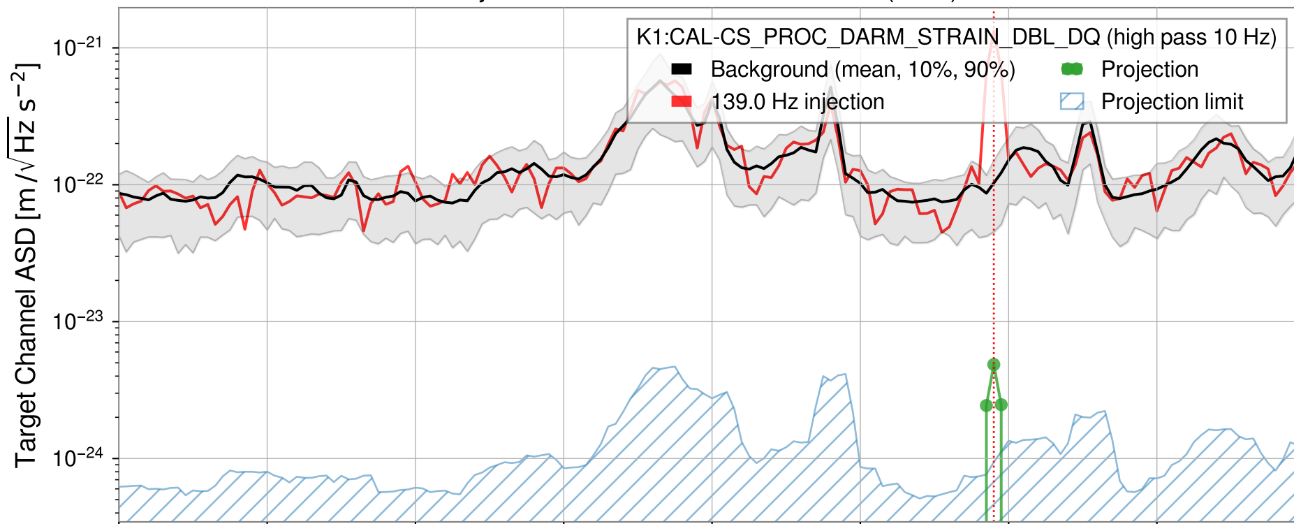
Injection from GPS1428961836.665 (8sec)
