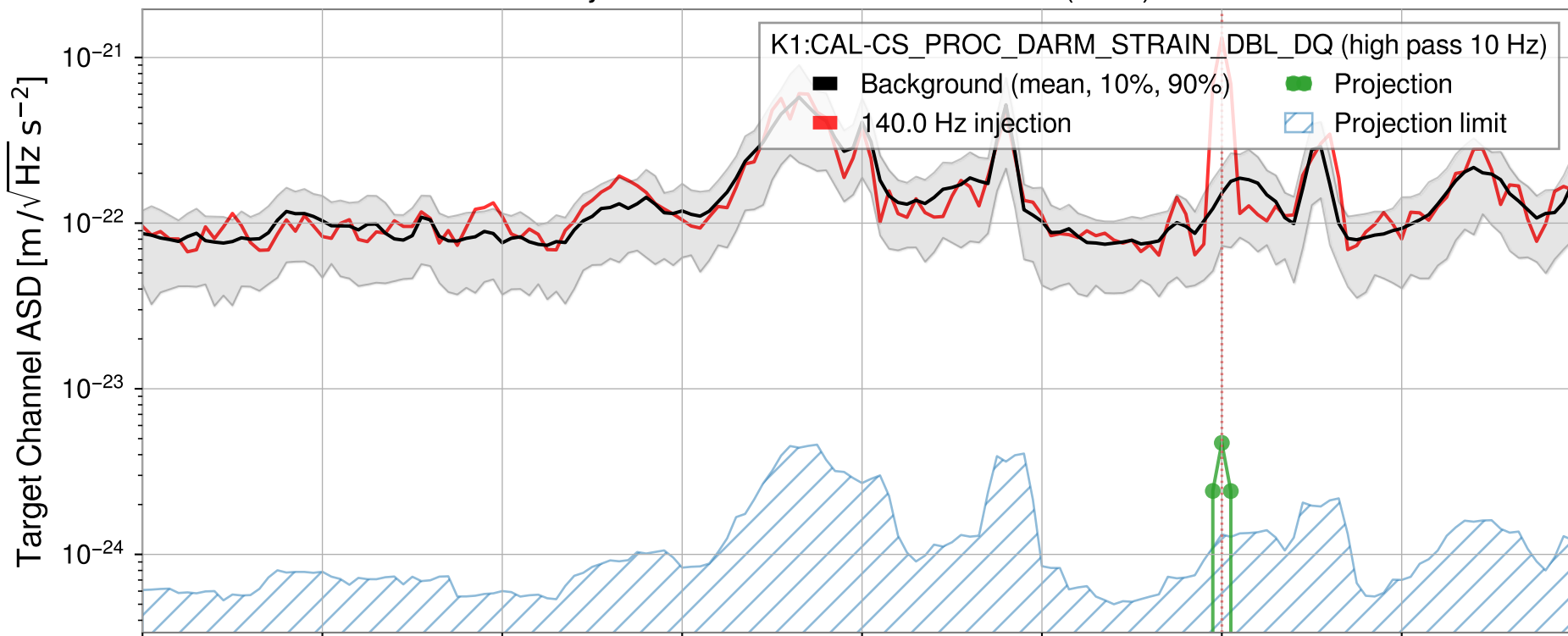
Injection from GPS1428961824.65 (8sec)
