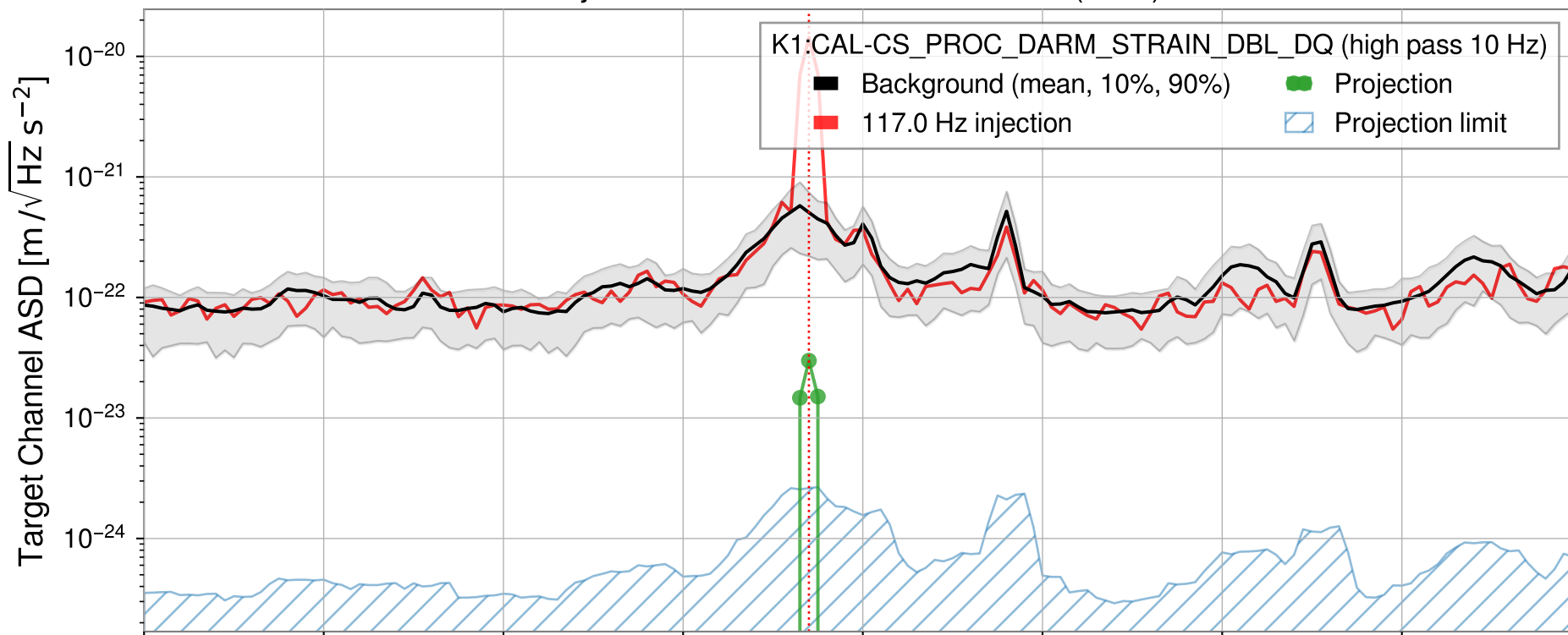
Injection from GPS1428962100.995 (8sec)
