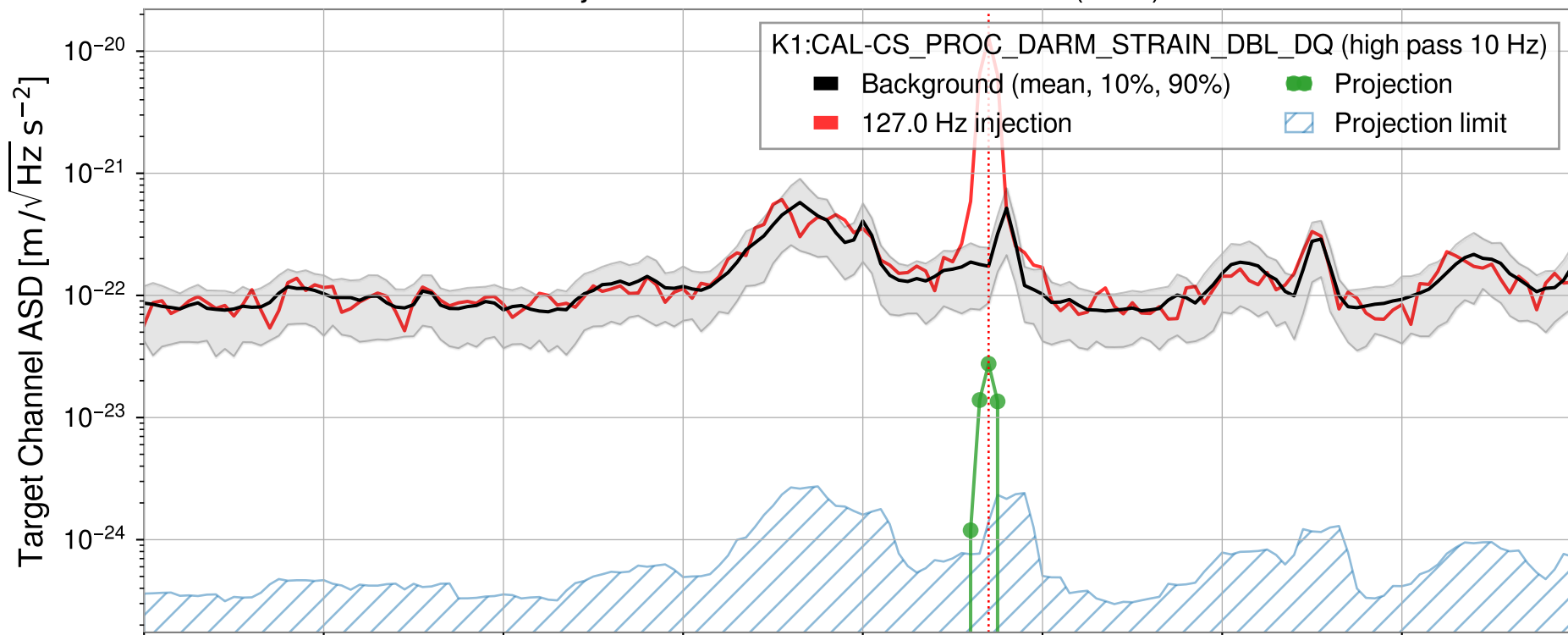
Injection from GPS1428961980.845 (8sec)
