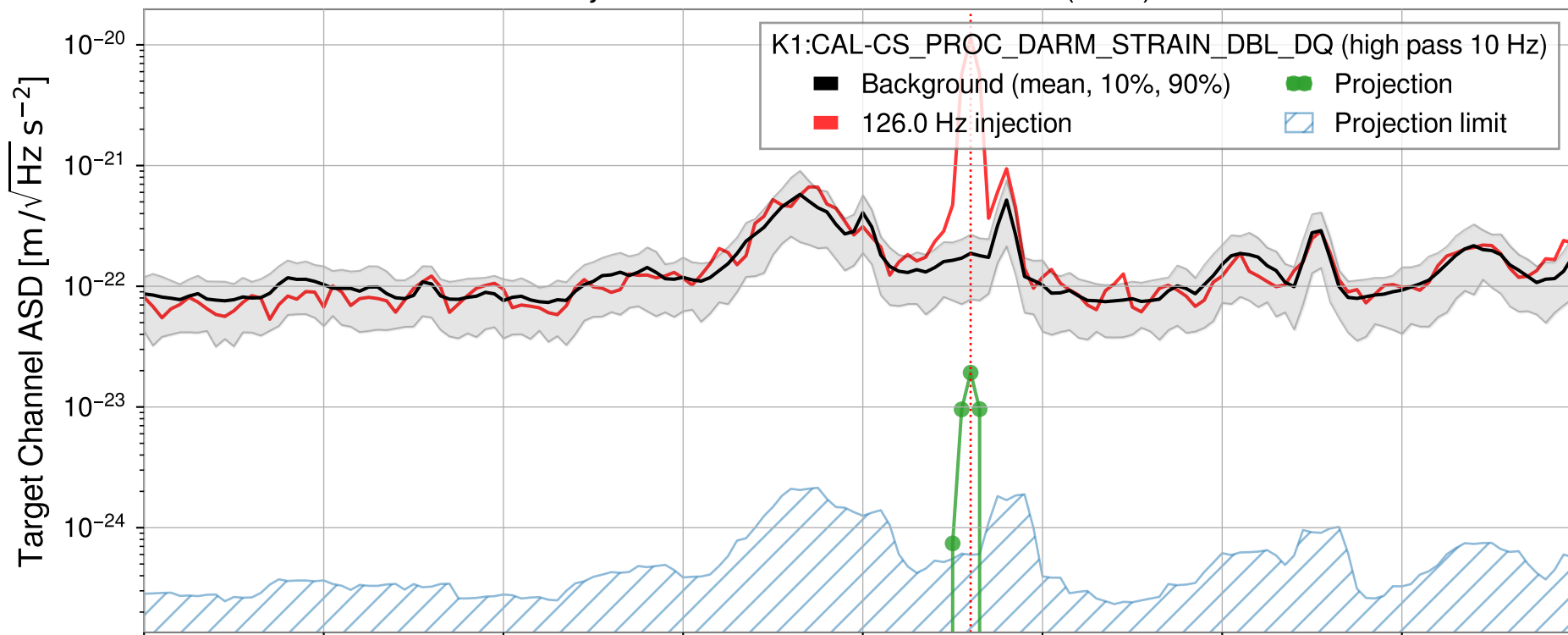
Injection from GPS1428961992.86 (8sec)
