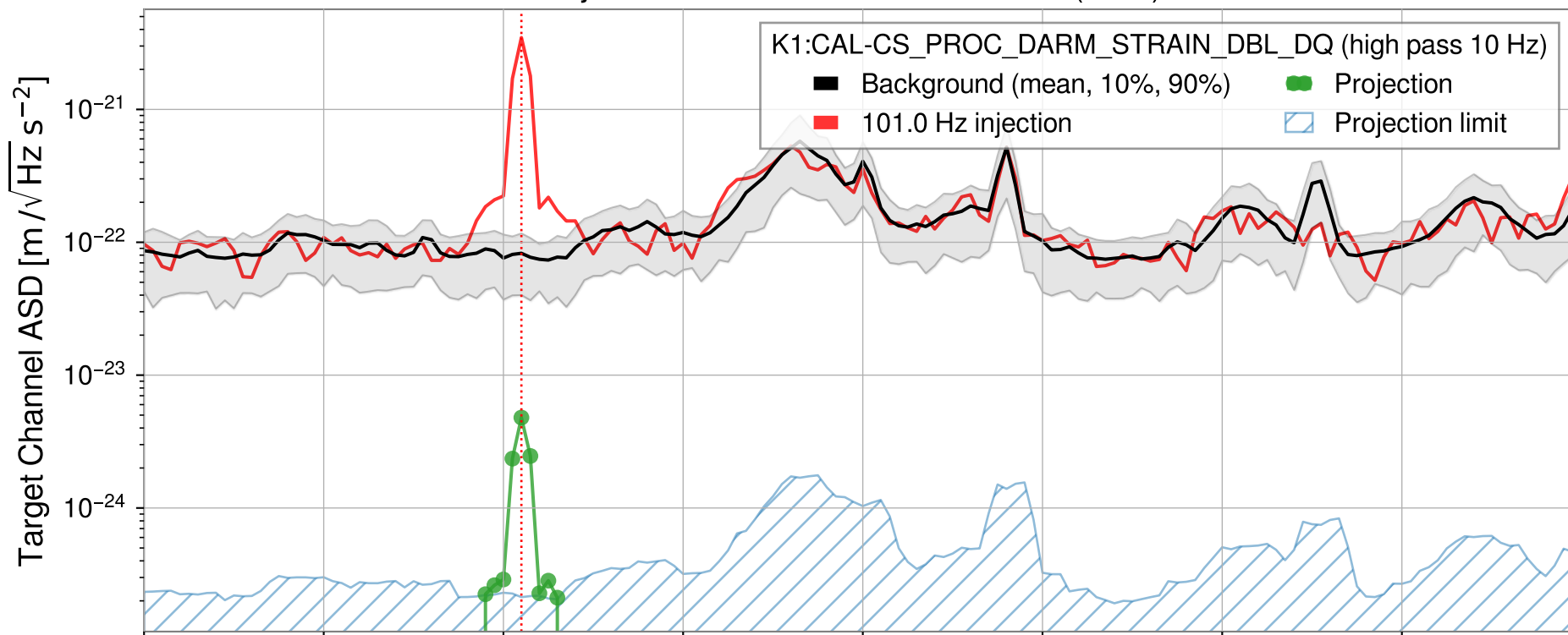
Injection from GPS1428962293.235 (8sec)
