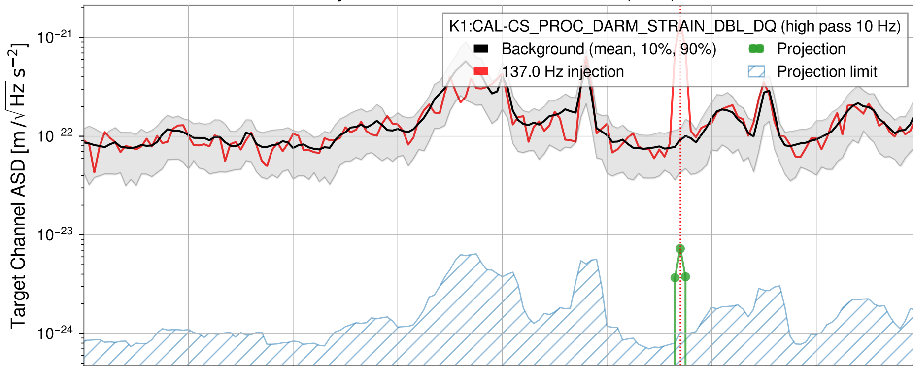
Injection from GPS1428961860.695 (8sec)
