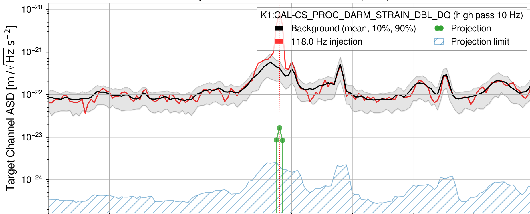
Injection from GPS1428962088.98 (8sec)
