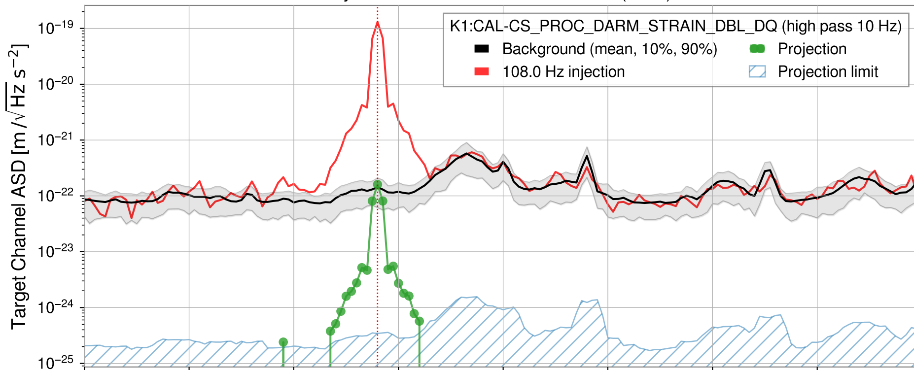
Injection from GPS1428962209.13 (8sec)
