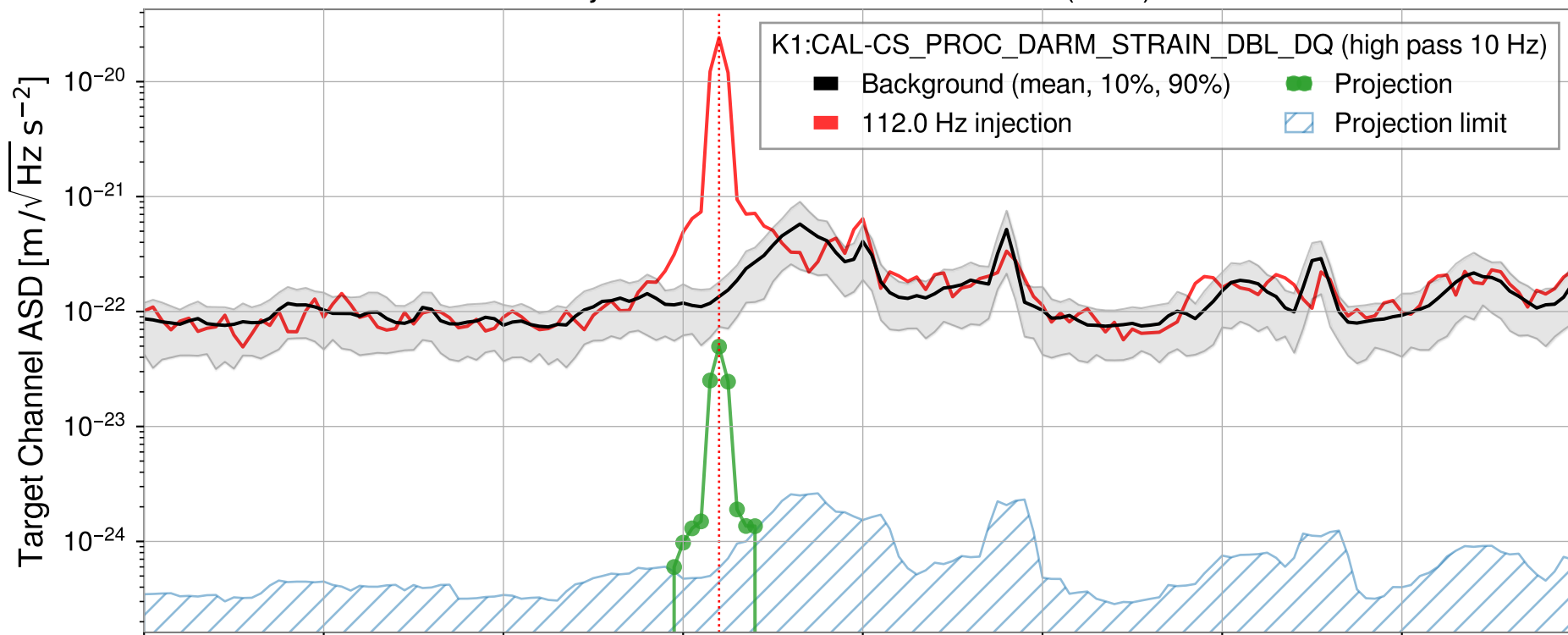
Injection from GPS1428962161.07 (8sec)
