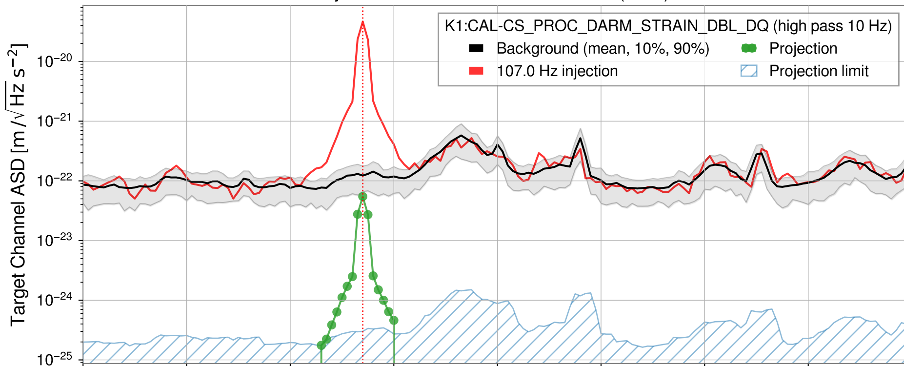
Injection from GPS1428962221.145 (8sec)
