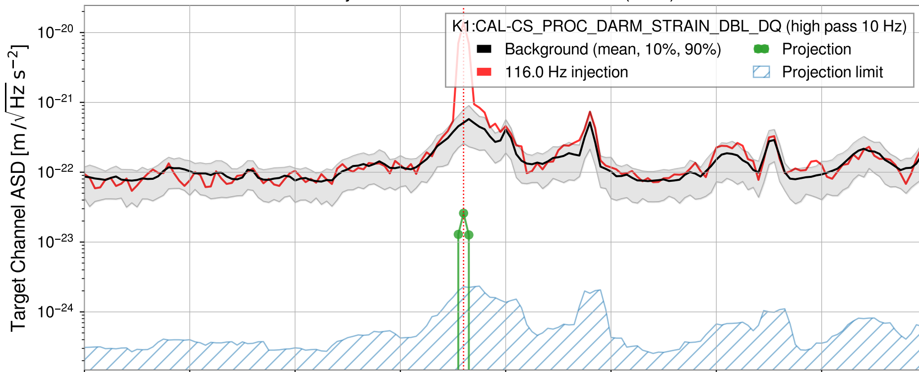
Injection from GPS1428962113.01 (8sec)
