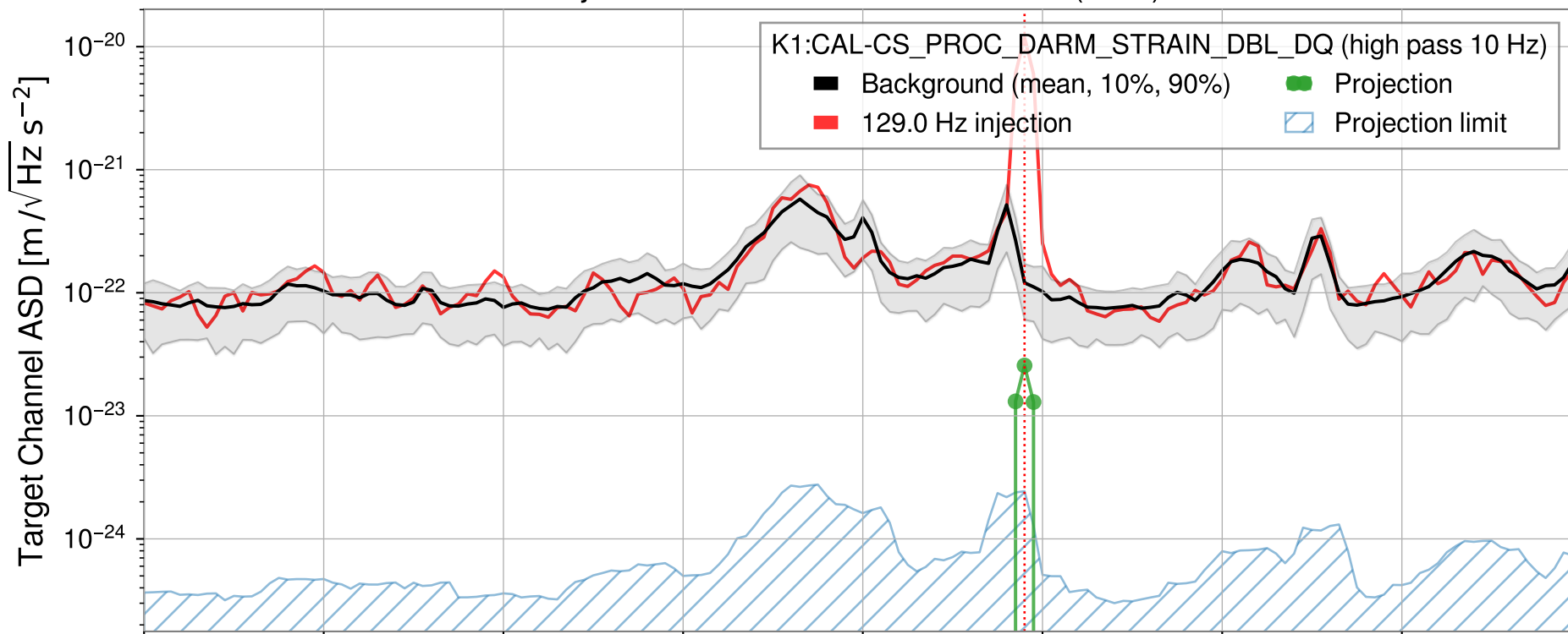
Injection from GPS1428961956.815 (8sec)
