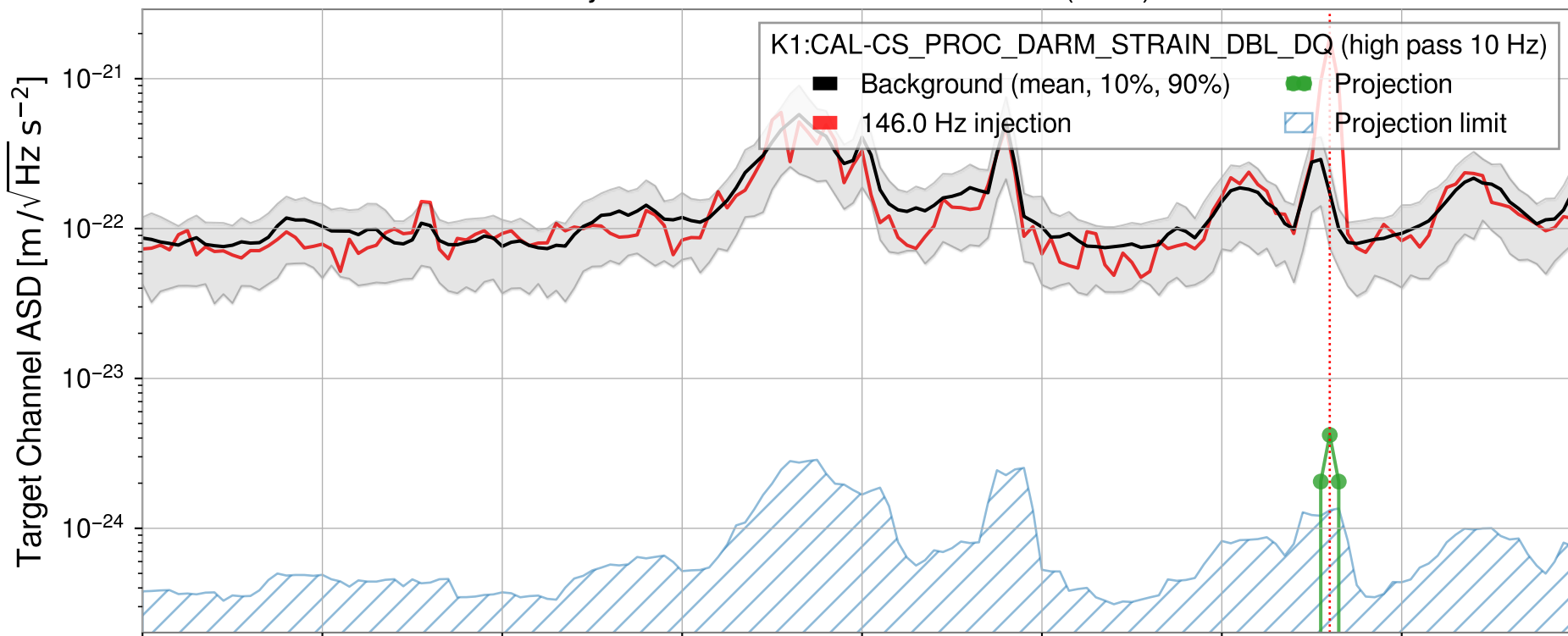
Injection from GPS1428961752.56 (8sec)
