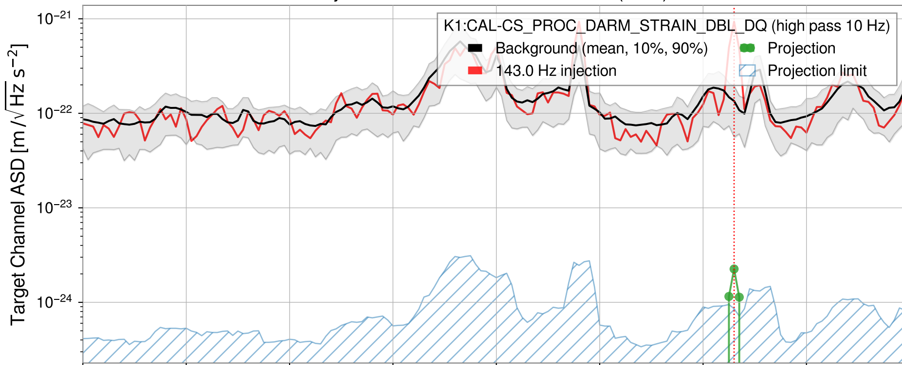
Injection from GPS1428961788.605 (8sec)
