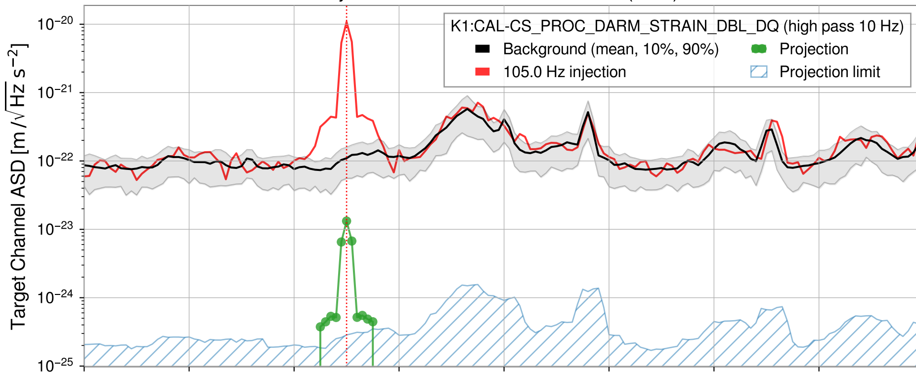
Injection from GPS1428962245.175 (8sec)
