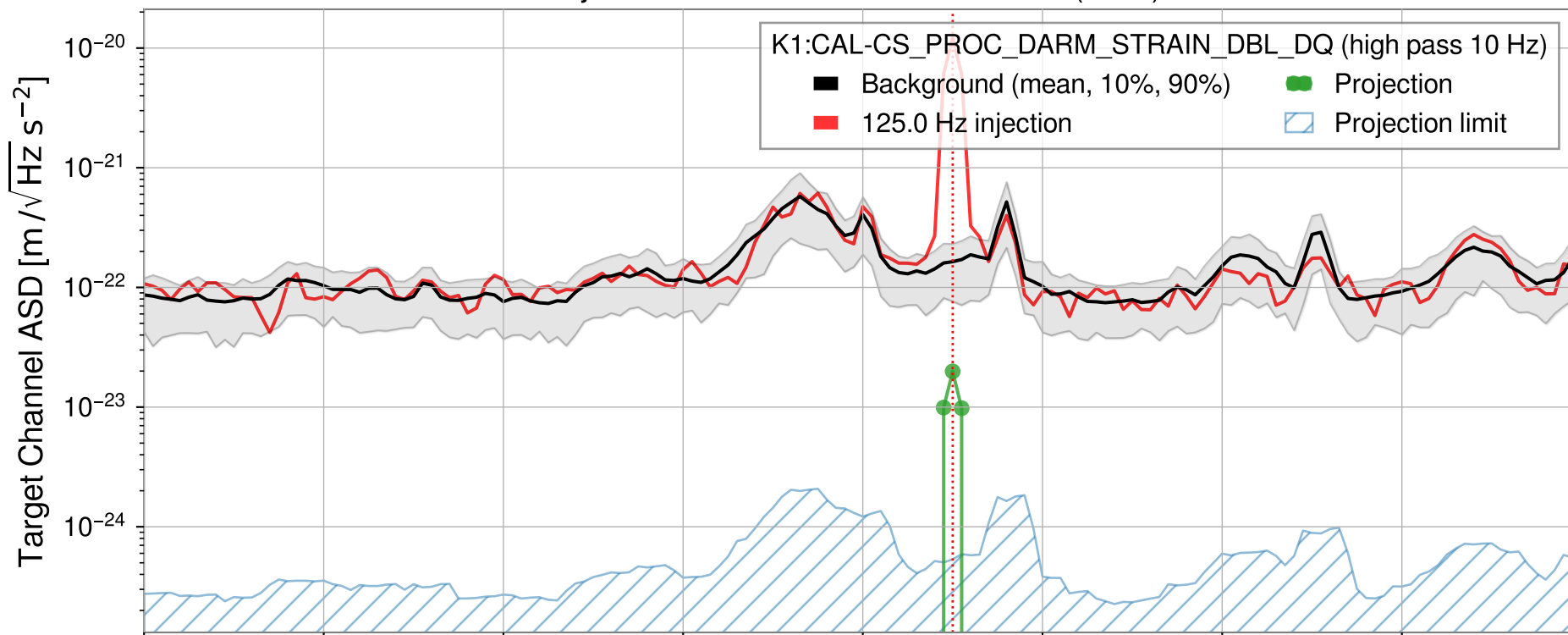
Injection from GPS1428962004.875 (8sec)
