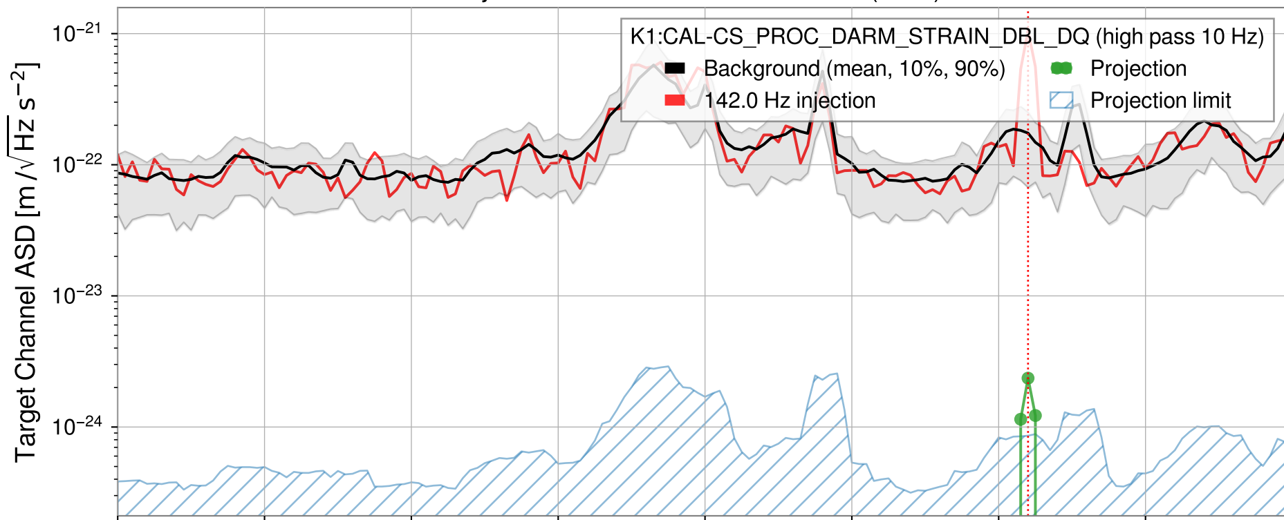
Injection from GPS1428961800.62 (8sec)
