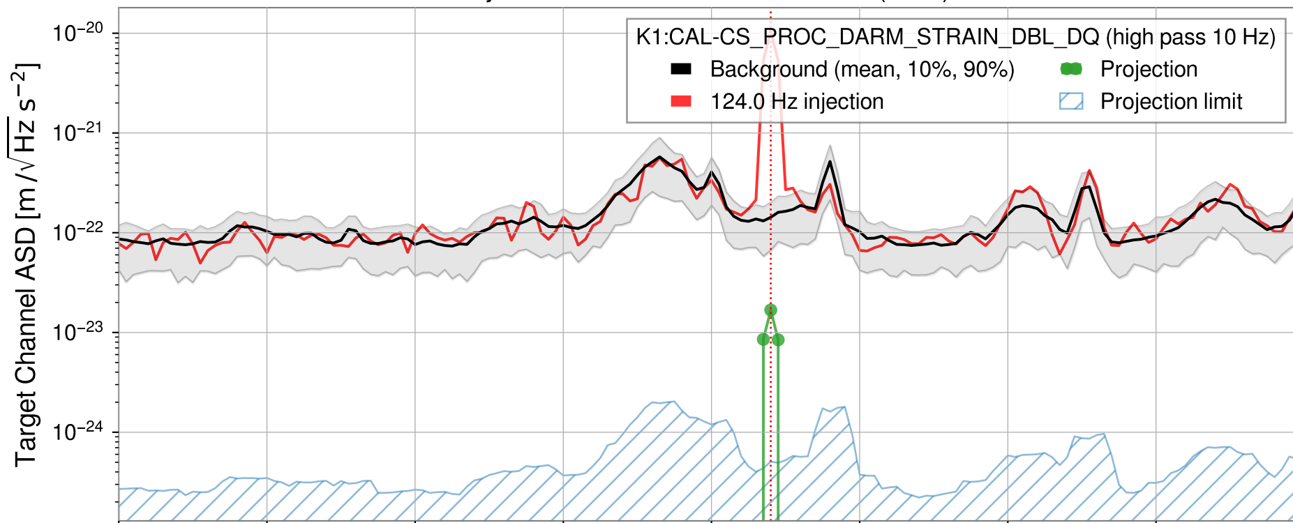
Injection from GPS1428962016.89 (8sec)
