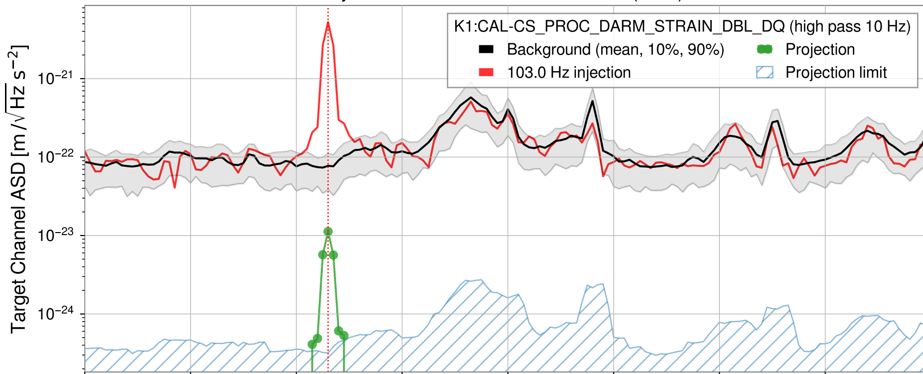
Injection from GPS1428962269.205 (8sec)
