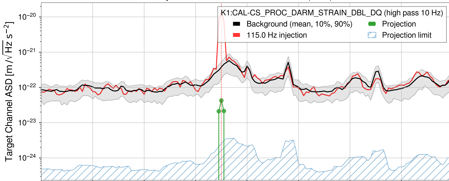
Injection from GPS1428962125.025 (8sec)
