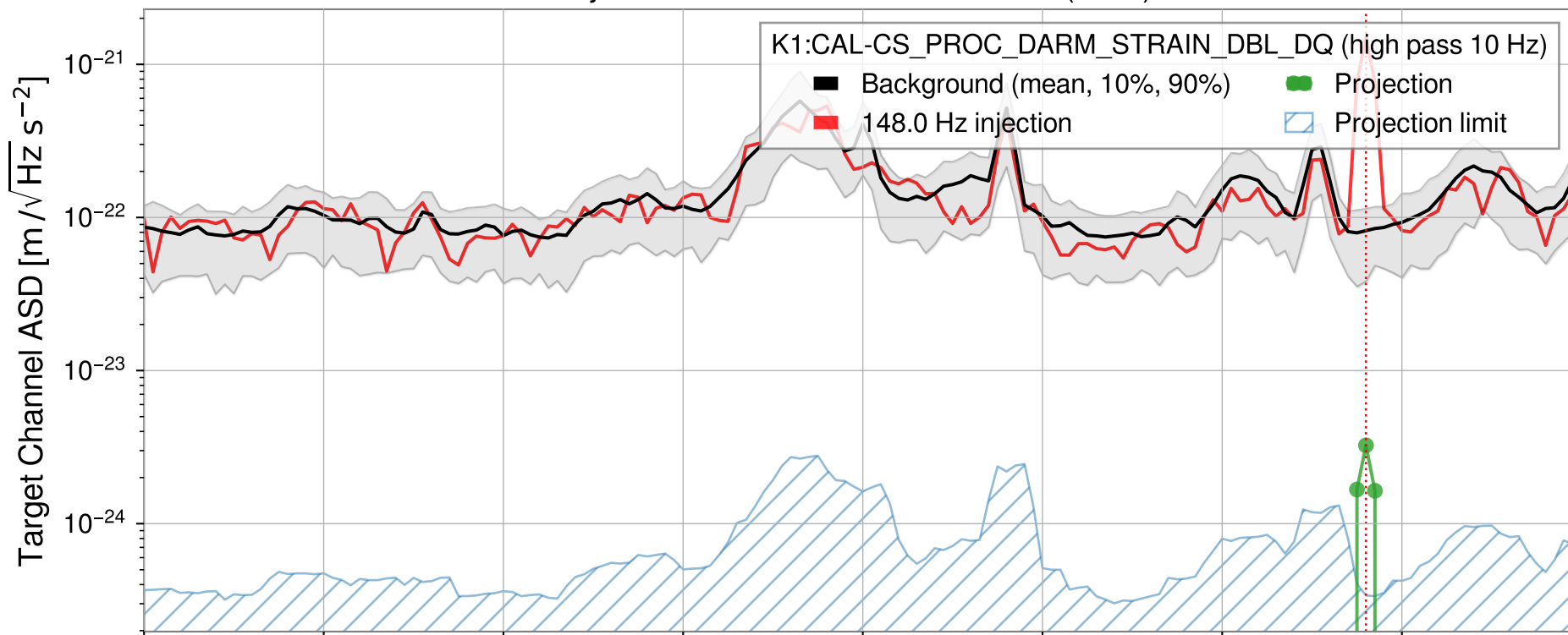
Injection from GPS1428961728.53 (8sec)
