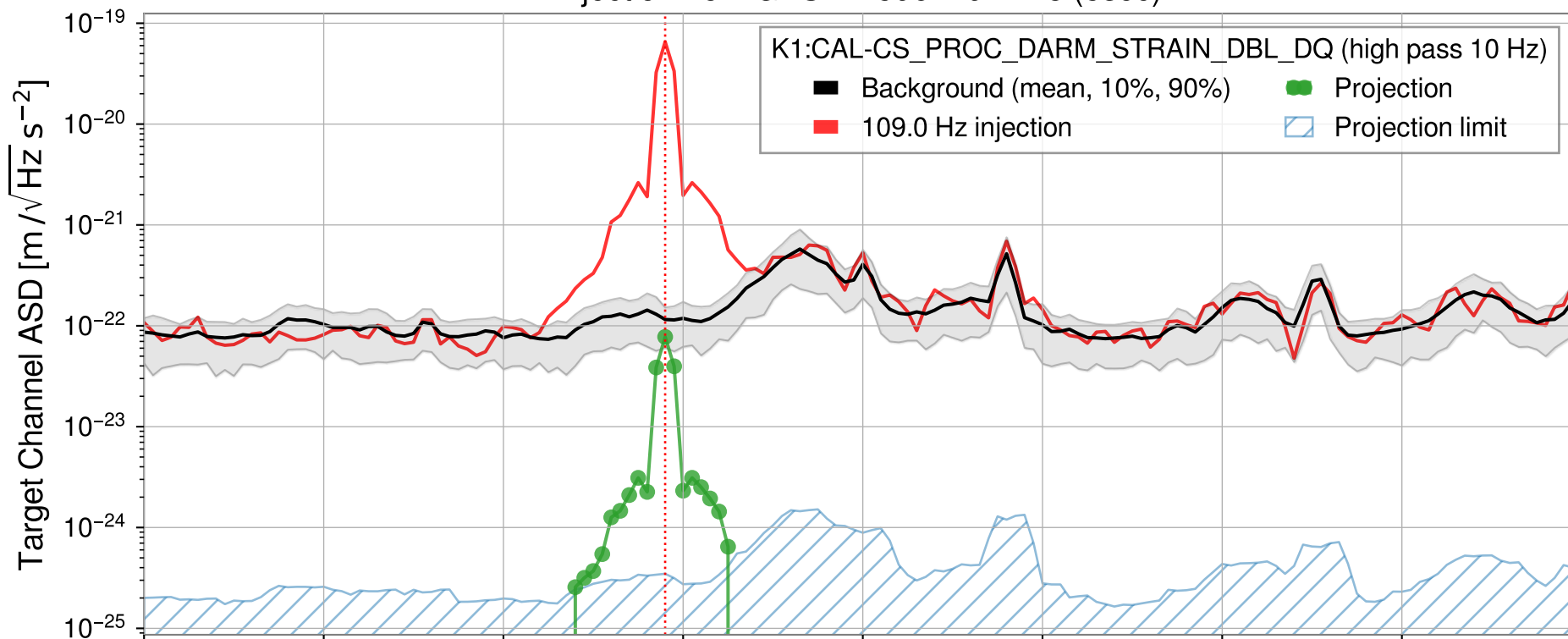
Injection from GPS1428962197.115 (8sec)
