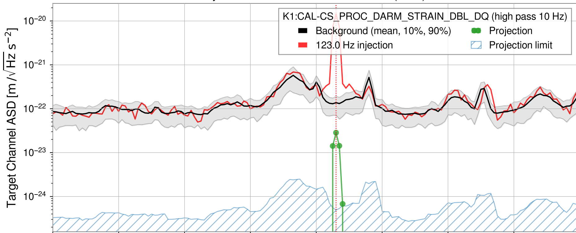
Injection from GPS1428962028.905 (8sec)
