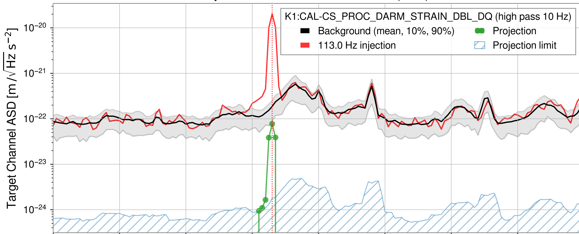
Injection from GPS1428962149.055 (8sec)
