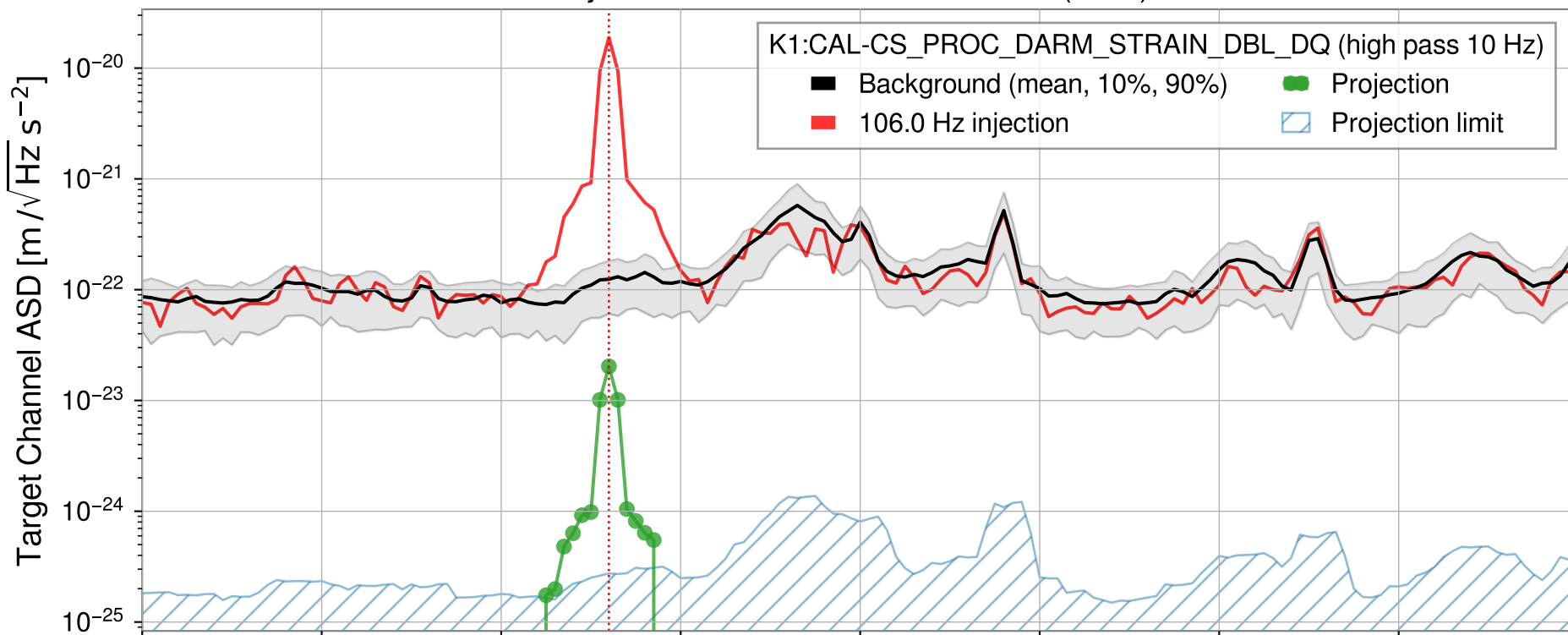
Injection from GPS1428962233.16 (8sec)
